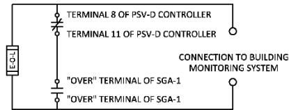
INERTING BYPASS SIGNAL WIRING DIAGRAM
